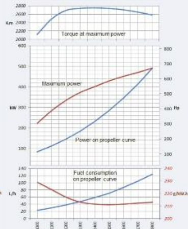
Rating P1 - 491 kW (668 hp) @ 1800 rpm
