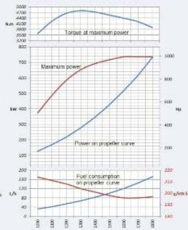
Rating P1 - 736 kW (1000 hp) @ 1800 rpm
