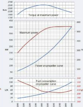
Rating P2 - 404 kW (550 hp) @ 1900 rpm
