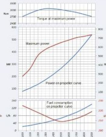
Rating P2 - 539 kW (733 hp) @ 1900 rpm
