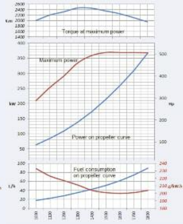
Rating P1 - 368 kW (500 hp) @ 1800 rpm
