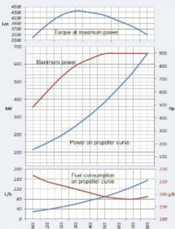
Rating P1 - 662 kW (900 hp) @ 1800 rpm
