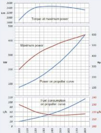
Rating P1 - 442 kW (600 hp) @ 1800 rpm
