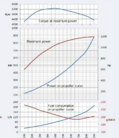
Rating P2 - 883 kW (1200 hp) @ 1950 rpm
