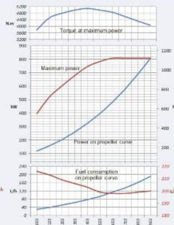
Rating P2 - 808 kW (1100 hp) @ 1900 rpm
