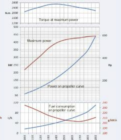
Rating P2 - 442 kW (600 hp) @ 1950 rpm
