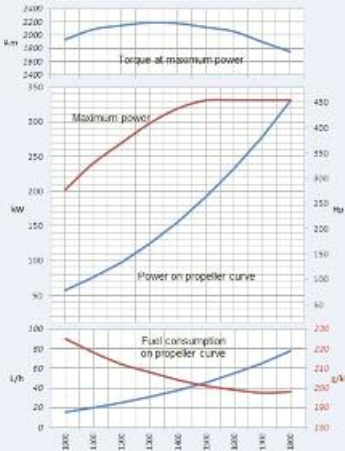
Rating P1 - 331 kW (450 hp) @ 1800 rpm
